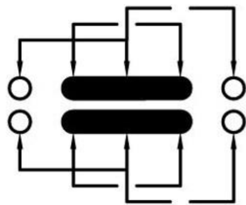
SCHEMATIC (NON-SHORTING)
